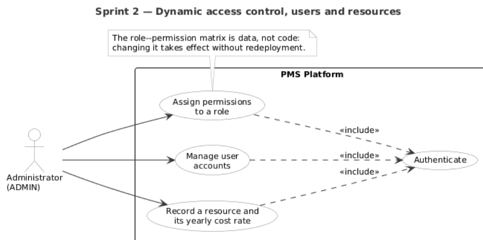
Figure 4.14: Use case diagram of sprint 2
